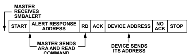
Figure 68. INT/ \overline{\text{INT}} Responds to SMBALERT ARA
