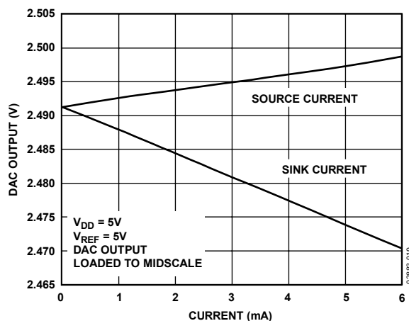
Figure 18. DAC V_{OUT} Source and Sink Current Capability
