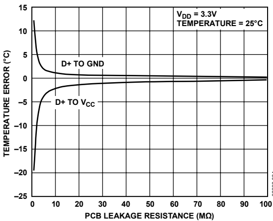
Figure 33. External Temperature Error vs. PCB Leakage Resistance
