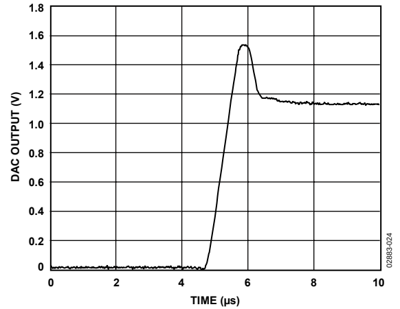
Figure 23. Exiting Power-Down to Midscale
