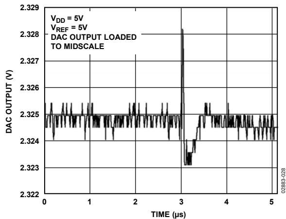
Figure 27. DAC-to-DAC Crosstalk
