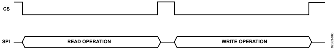
Figure 67. SPI—Correct Use of \overline{CS} during SPI Communication
