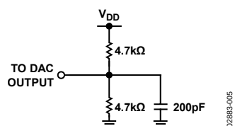
Figure 5. Load Circuit for DAC Outputs
