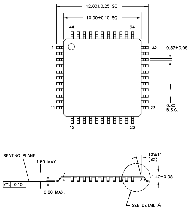
Figure 9. 44-pin TQFP
