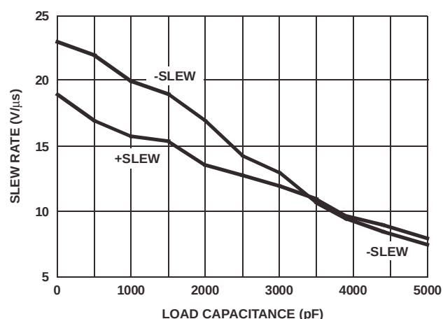
FIGURE 9. SLEW RATE vs LOAD CAPACITANCE
