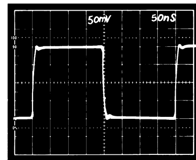
Figure 20c. Noninverting Small Signal Pulse Response
