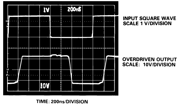
Figure 26. Overdrive Recovery
