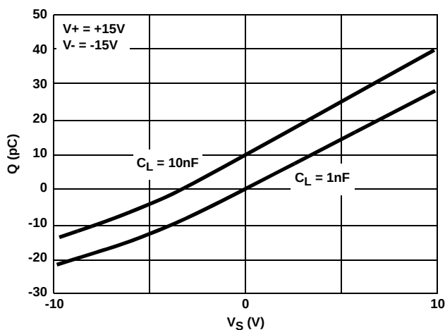
FIGURE 13. CHARGE INJECTION vs SOURCE VOLTAGE
