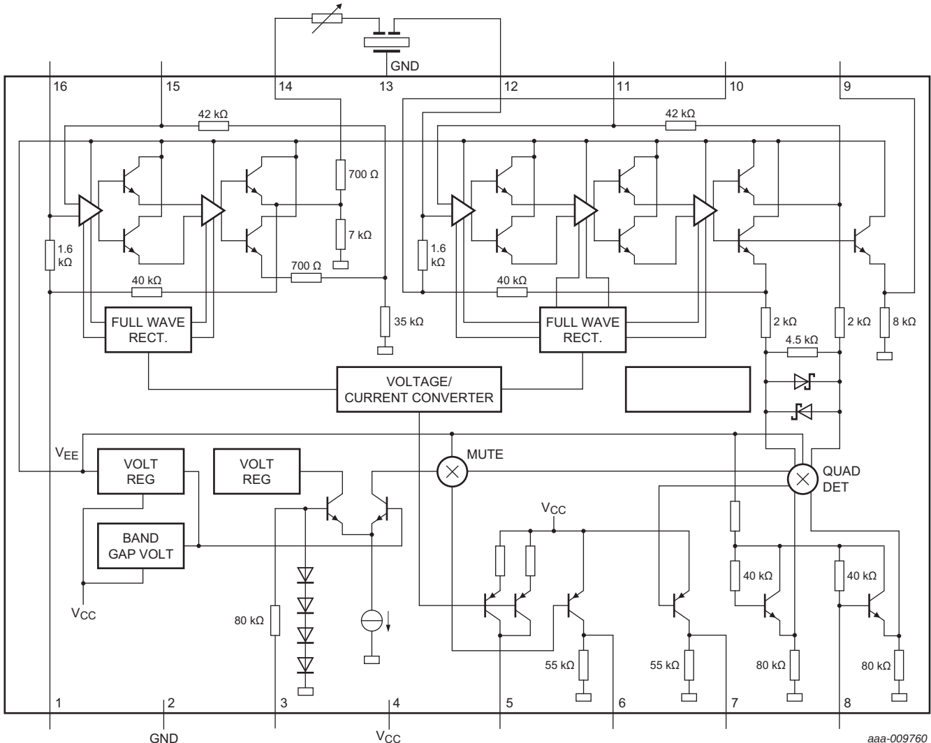
Fig 4. Equivalent circuit
