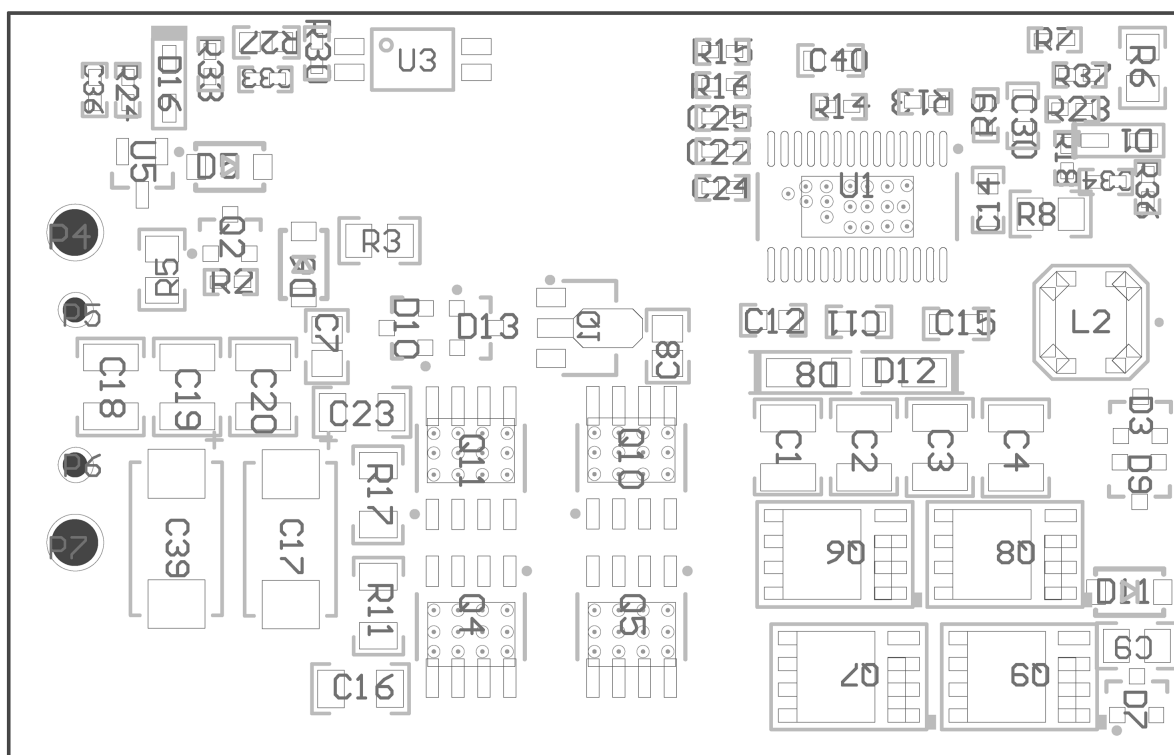
Figure 11. Bottom Side Assembly
