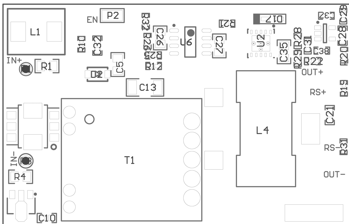
Figure 10. Top Side Assembly
