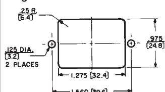
Front Mount EAC305 Figure 2
