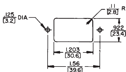
Front Mount EAC225 Figure 5
