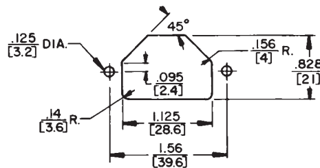
Rear Mount EAC323 Figure 6
