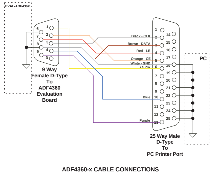
ADF4360-x CABLE CONNECTIONS
