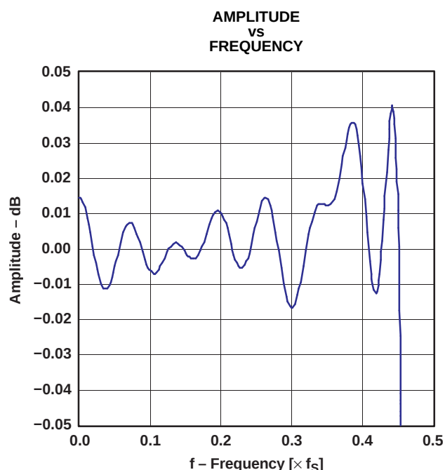
Figure 2. Pass-Band Ripple
