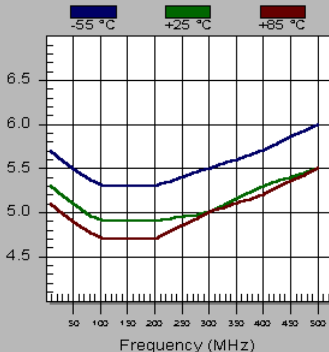
TM6507 Noise Figure (dB)
