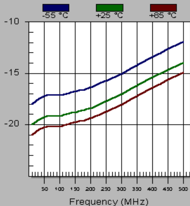
TM6507 Reverse Isolation (dB)
