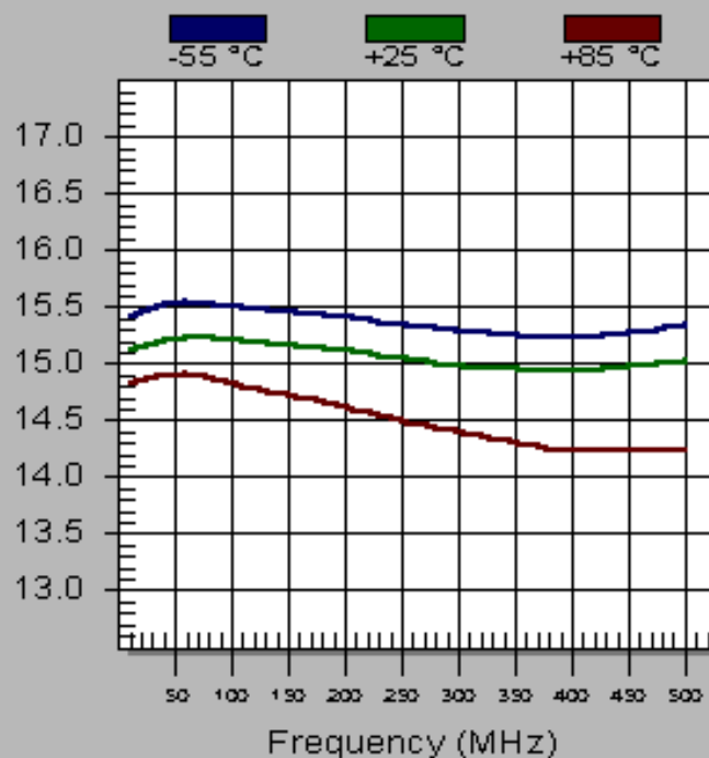
TM6507 Gain (dB)
