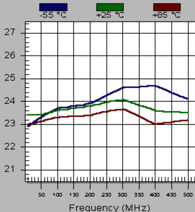
TM6507 1 dB Comp Point (dBm)
