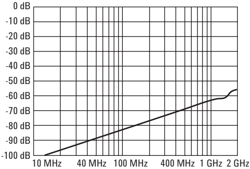
34942A typical initial crosstalk
