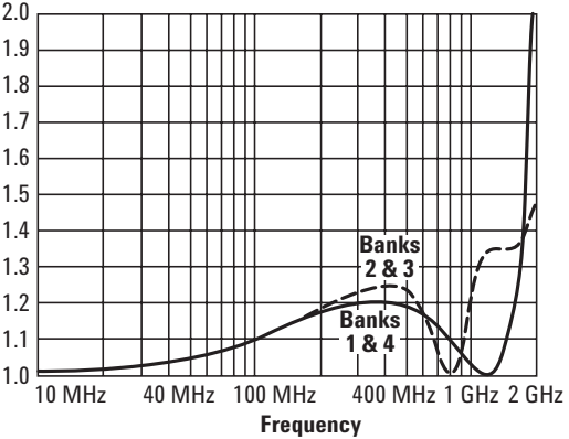
34942A typical initial VSWR
