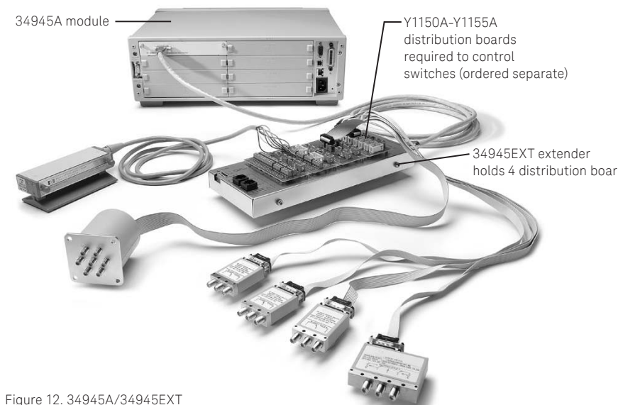
Figure 12. 34945A/34945EXT microwave switch/attenuator driver
