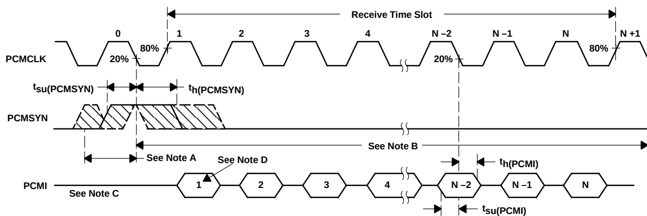
Figure 1. Transmit Timing Diagram (2.048 MHz)
