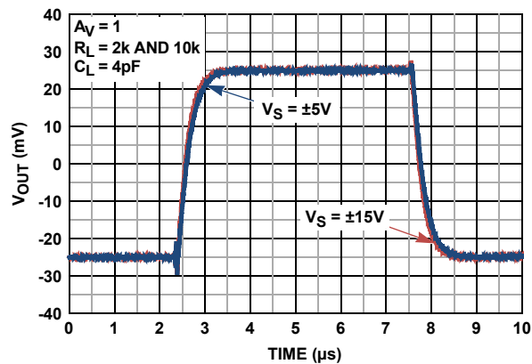
FIGURE 28. CHARACTERIZED SMALL SIGNAL TRANSIENT RESPONSE vs R_L , V_S = \pm 0.9V, \pm 2.5V
