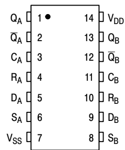
PIN ASSIGNMENT
