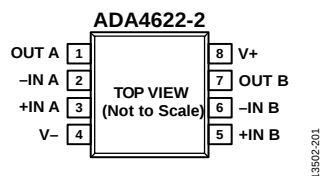
Figure 5. 8-Lead SOIC Pin Configuration, ADA4622-2
