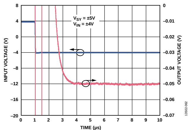
Figure 66. Negative Settling Time, A_V = -10 , V_{SV} = \pm 5V
