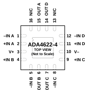
NOTES 1. NIC = NOT INTERNALLY CONNECTED. 2. THE EXPOSED PAD MUST BE CONNECTED TO V+. 13502-407 Figure 7. 16-Lead LFCSP Pin Configuration, ADA4622-4
