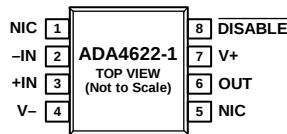
Figure 3. 8-Lead SOIC Pin Configuration, ADA4622-1
