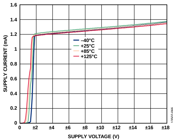
Figure 70. Supply Current ( I_{SV} ) vs. Supply Voltage ( V_{SV} ) for Various Temperatures
