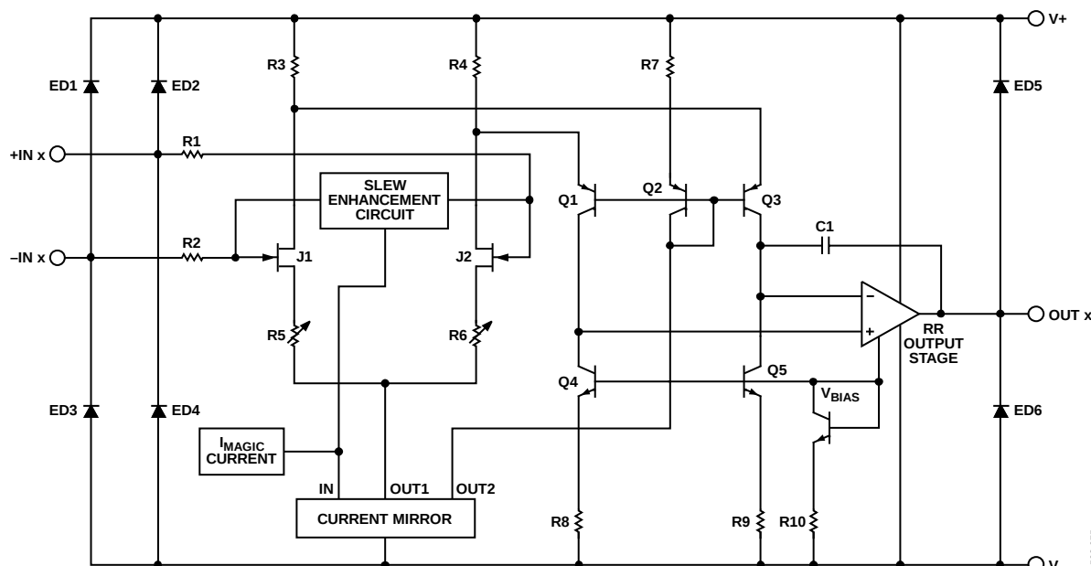
Figure 80. Simplified Circuit Diagram
