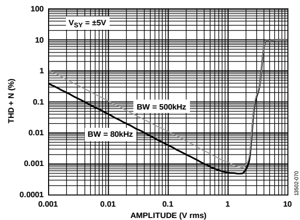
Figure 74. THD + N vs. Amplitude, V_{SV} = \pm 5\text{ V}
