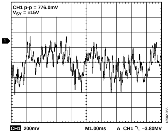
Figure 69. 0.1 Hz to 10 Hz Noise, V_{SV} = \pm 15\text{ V}
