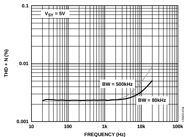
Figure 78. THD + N vs. Frequency, V_{SY} = 5\text{ V}
