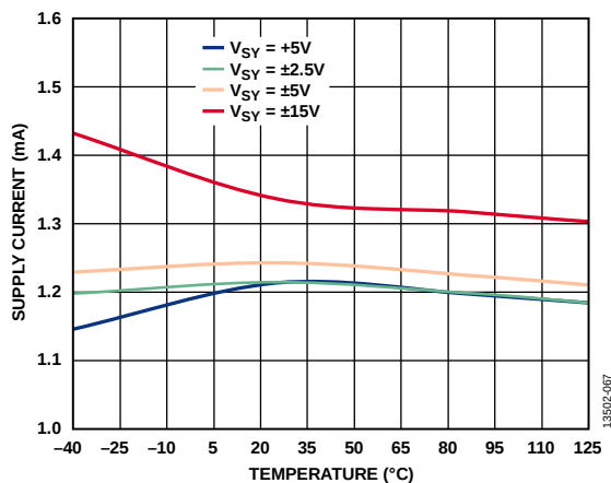
Figure 71. Supply Current ( I_{SV} ) vs. Temperature for Various Supply Voltages
