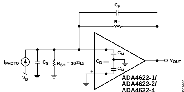
Figure 94. Wideband Photodiode Preamplifier
