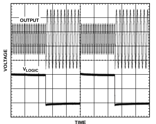
Figure 101. Multiplexed Output
