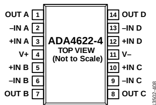
Figure 8. 14-Lead SOIC Pin Configuration, ADA4622-4
