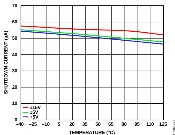
Figure 79. Shutdown Current vs. Temperature
