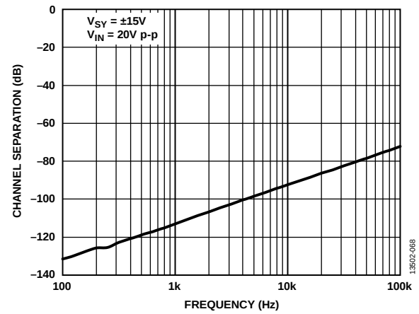
Figure 72. Channel Separation vs. Frequency, V_{SV} = \pm 15\text{ V}
