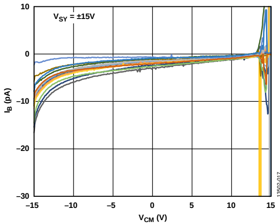
Figure 21. Input Bias Current ( I_B ) vs. Input Common-Mode Voltage ( V_{CM} ), V_{SY} = \pm 15\text{ V}
