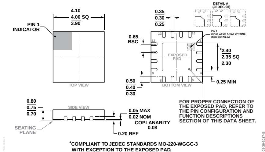
Figure 108. 16-Lead Lead Frame Chip Scale Package [LFCSP] 4 mm x 4 mm Body and 0.75 mm Package Height (CP-16-20) Dimensions shown in millimeters
