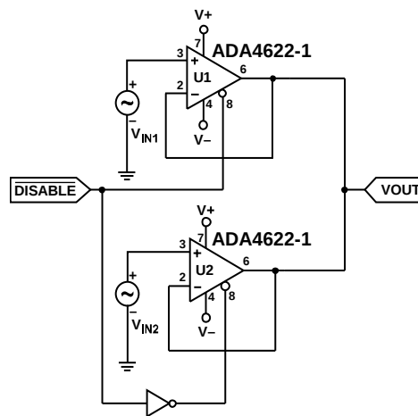
Figure 100. Multiplexed Input Circuit
