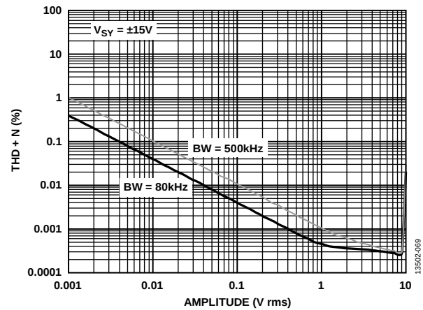
Figure 73. THD + N vs. Amplitude, V_{SV} = \pm 15\text{ V}
