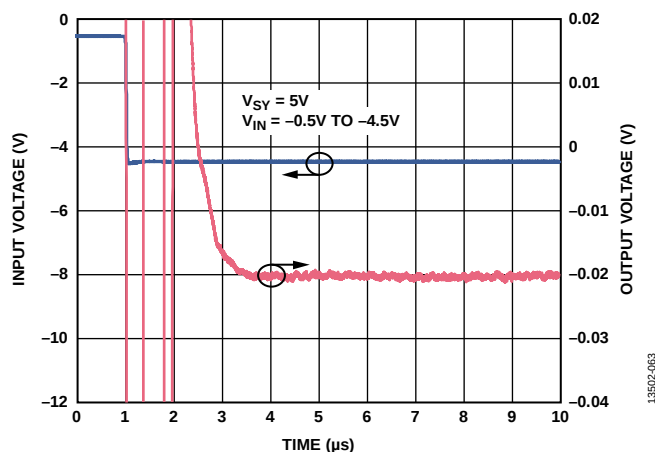
Figure 67. Negative Settling Time, A_V = -10 , V_{SV} = 5V
