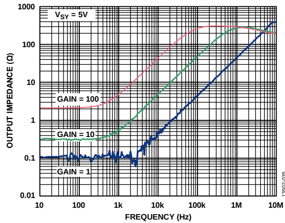
Figure 39. Output Impedance vs. Frequency, V_{SV} = 5\text{ V}
