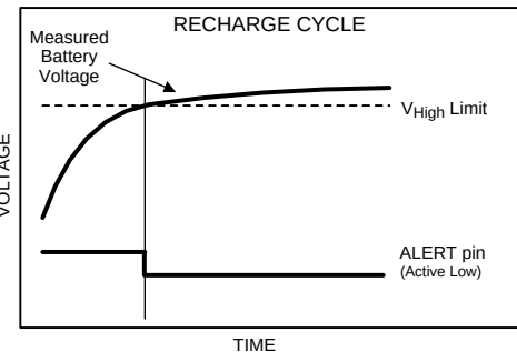
Figure 39. Recharge Cycle
