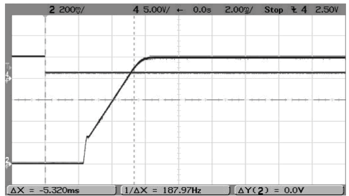
On/Off Enable Startup ( V_{IN} = 5V , V_{OUT} = 1.0V , I_{OUT} = 6A , Load=0) Trace 4=Enable, Trace2=Vout
