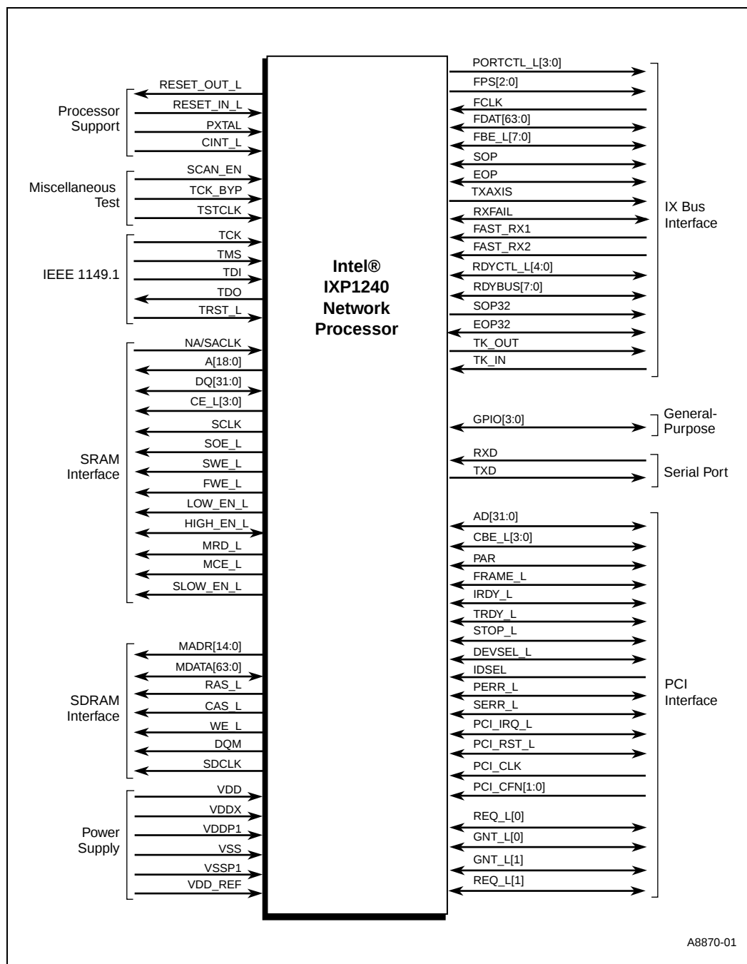
Figure 6. Pinout Diagram
