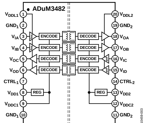
Figure 3. ADuM3482
