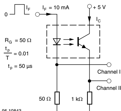
Fig. 2 - Test Circuit, Saturated Operation
