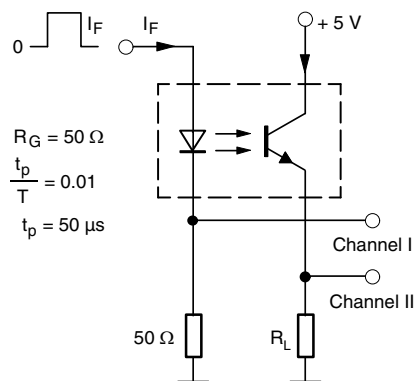
Fig. 1 - Test Circuit, Non-Saturated Operation
