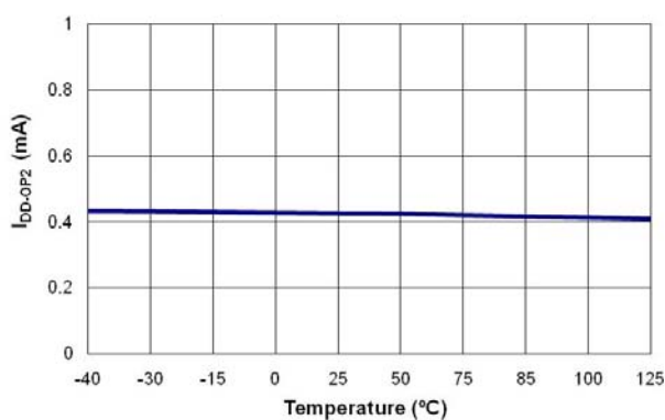
Figure 8. Operating Current ( I_{DD-OP2} ) vs. Temperature
