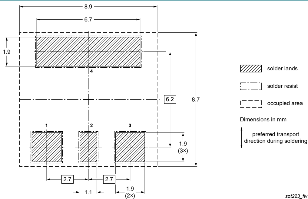
Fig. 14. Wave soldering footprint for SC-73 (SOT223)
