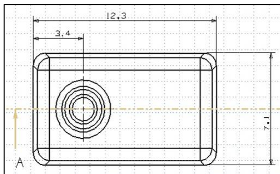
Figure 6.4 Mechanical drawing: Upside of tube connection (type A and type B)
