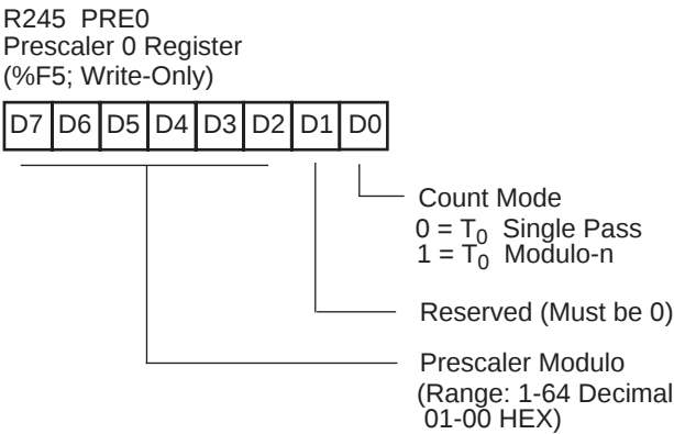
Figure 70. Prescaler 0 Register
