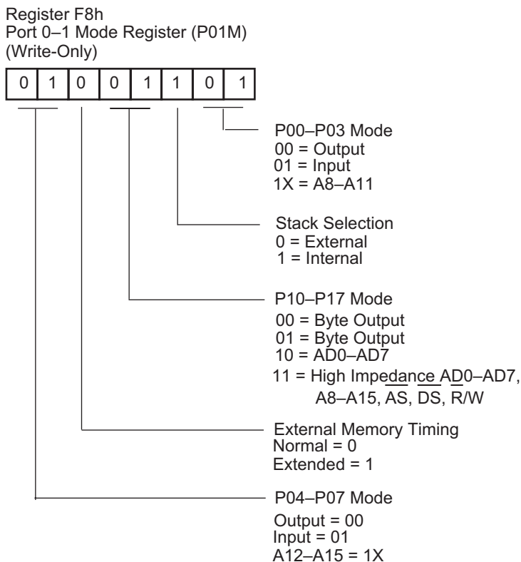
Figure 54. Port 0/1 Reset
