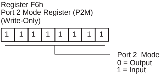
Figure 55. Port 2 Reset
