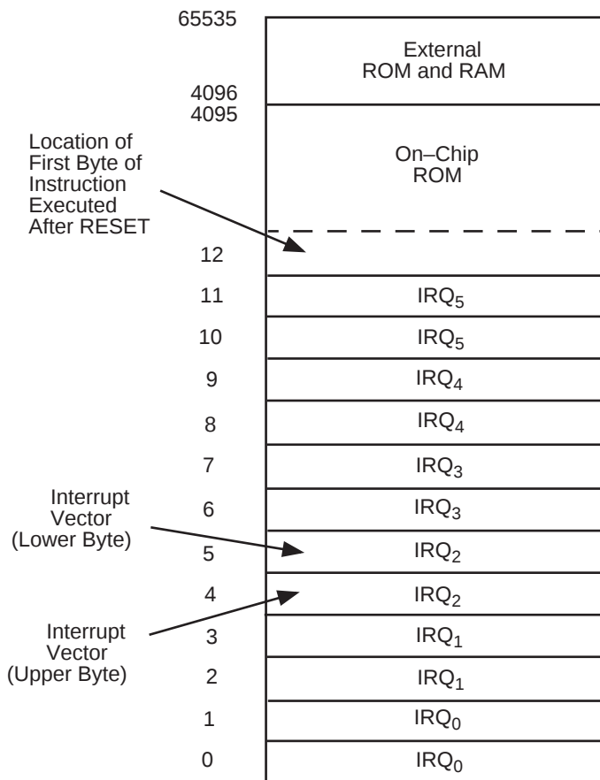
Figure 8. Z8 Program Memory Map
