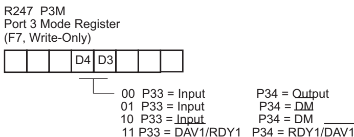
Figure 37. Handshake Operation
