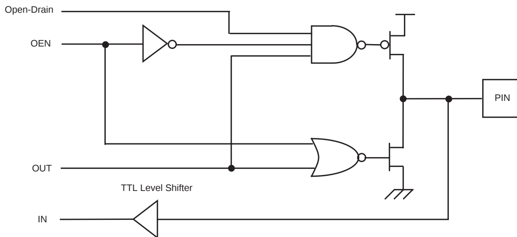
Figure 40. Port 2 Configuration with TTL Level Shifter
