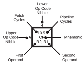
Figure 134. Op Code Map
