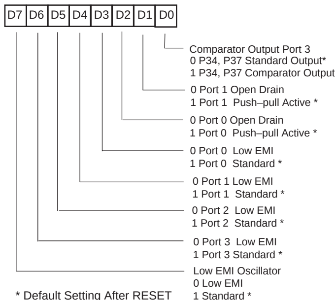
Figure 62. Port Configuration Register (Write-Only)
