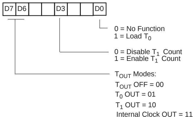
Figure 76. Timer Mode Register (T OUT Operation)
