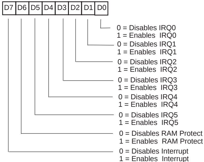
Register FBh Interrupt Request Register (IMR) (Read/Write)
