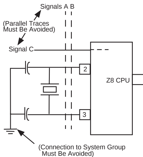
Figure 17. Circuit Board Design Rules
