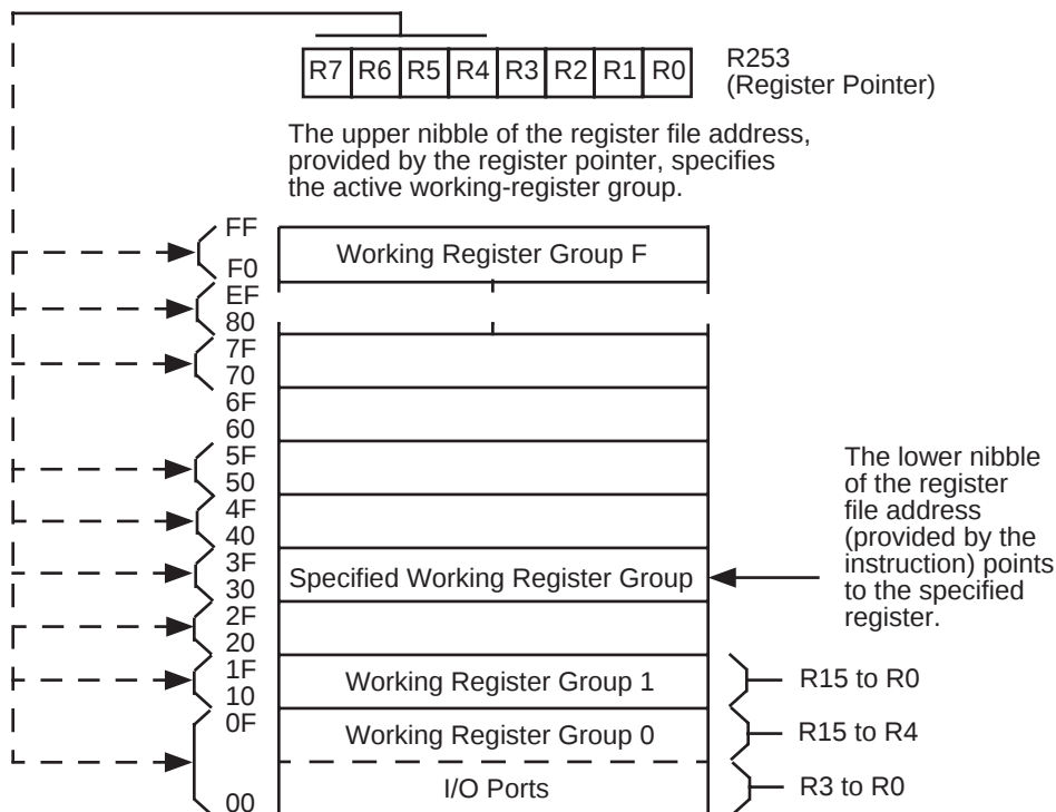
Figure 5. Register Pointer
