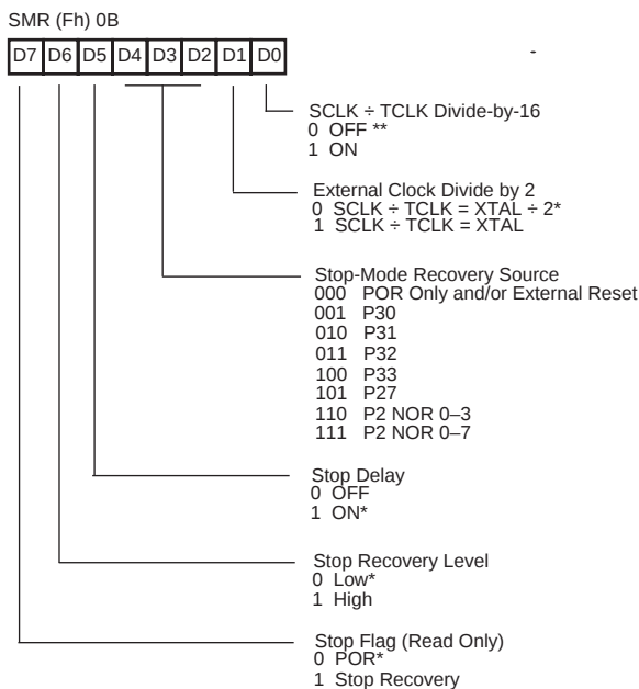
Figure 103. Stop-Mode Recovery Register (Write-Only Except Bit D7, Which Is Read-Only)
