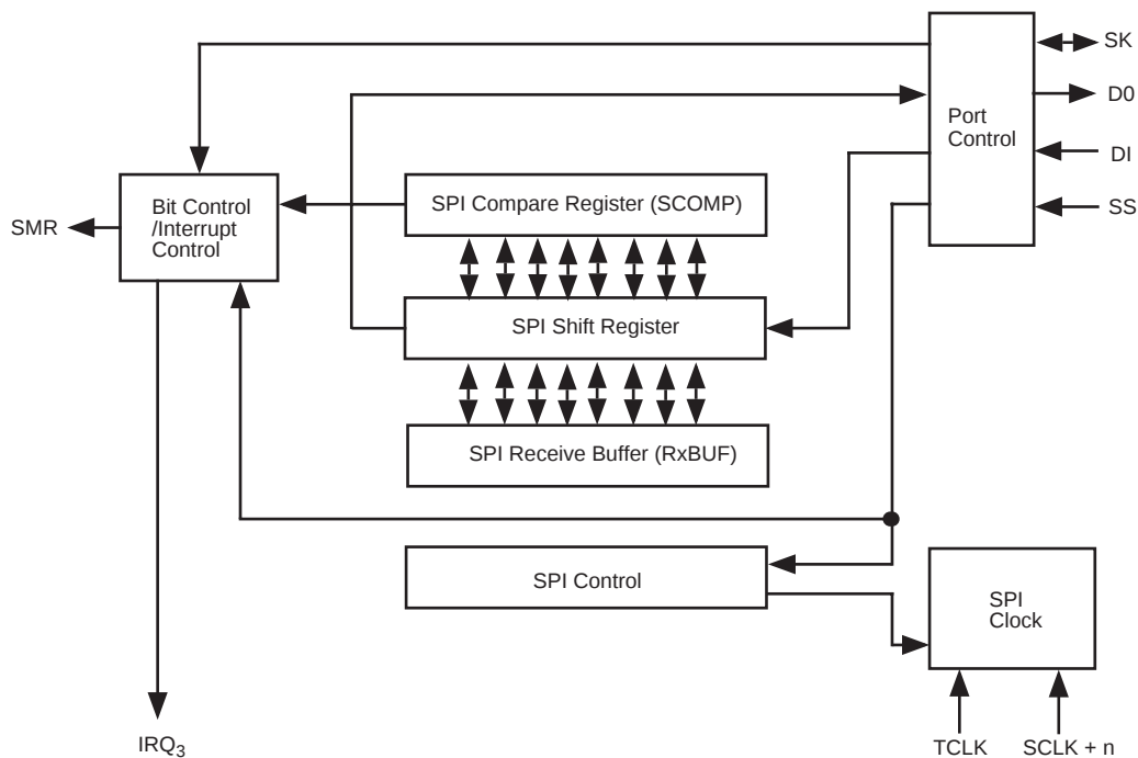
Figure 119. SPI Logic
