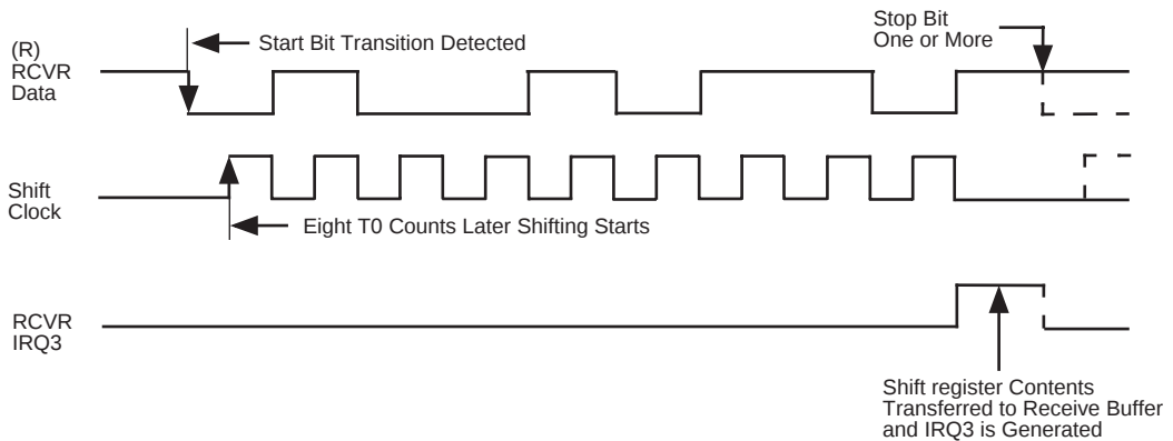
Figure 110. Receiver Timing
