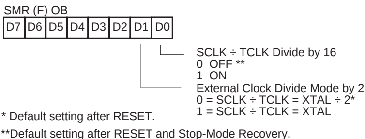
Figure 13. Stop-Mode Recovery Register (Write-Only Except D7, Which is Read-Only)
