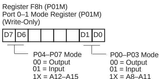
Figure 32. Port 0 I/O Operation
