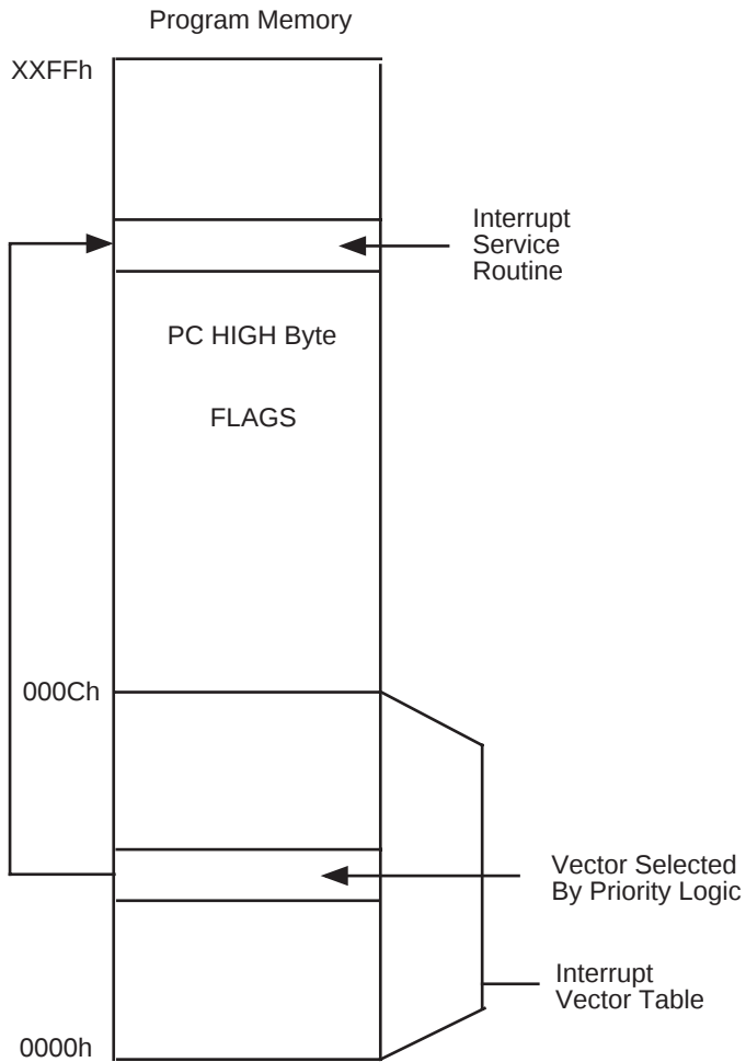
Figure 101. Interrupt Vectoring
