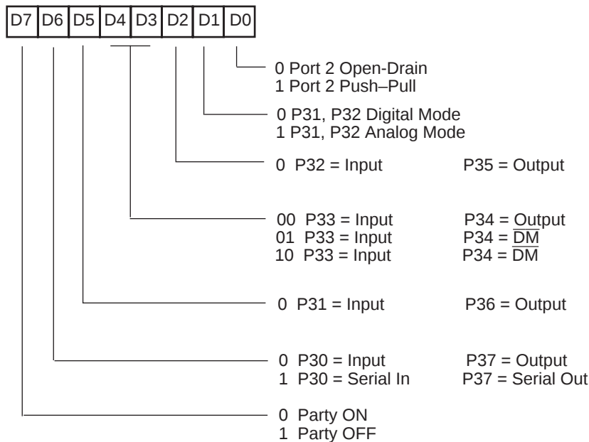
Register F7h Port 3 Mode Register (Write-Only)
