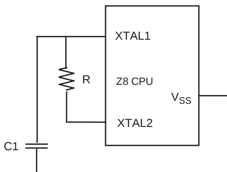
Figure 21. RC Clock
