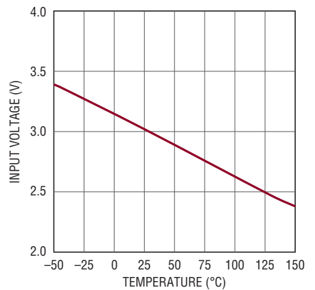
Minimum Input Voltage to Switch
