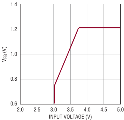
V_{\text{FB}} Regulation Voltage
