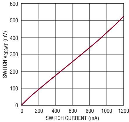
Switch V_{\text{CESAT}}
