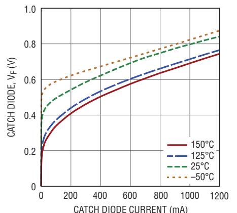
Catch Diode Forward Voltage
