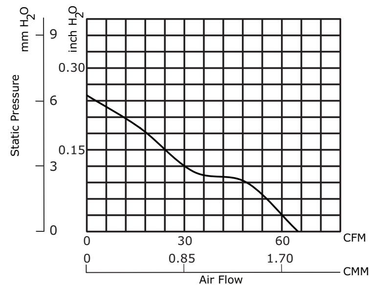
CFM-9225V-339-420
