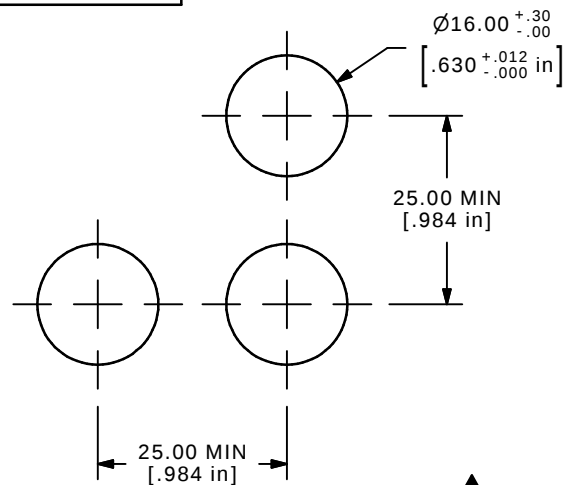
PANEL MOUNTING
