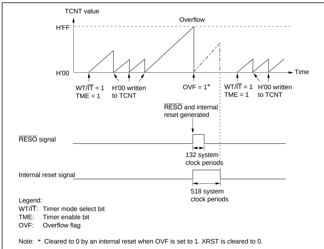
Figure 14.3 Operation in Watchdog Timer Mode ( \text{RST}/\overline{\text{NMI}} = 1 )
