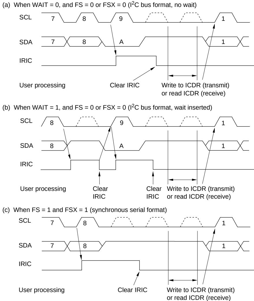
Figure 16.12 IRIC Setting Timing and SCL Control
