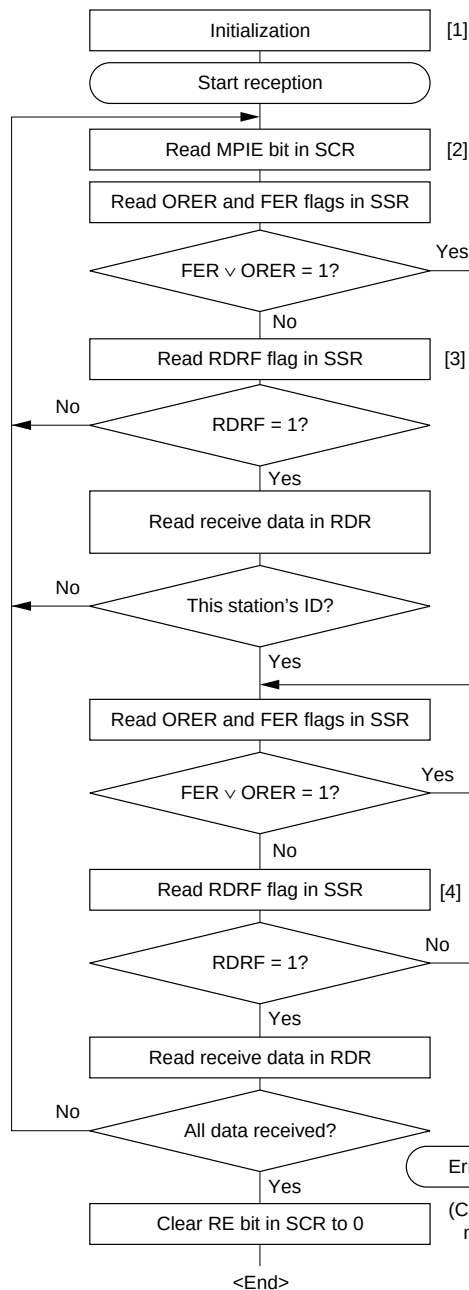
Figure 15.12 Sample Multiprocessor Serial Reception Flowchart
