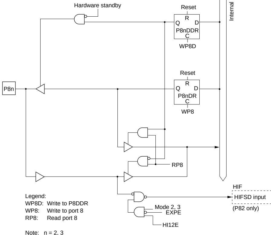
Figure C.25 Port 8 Block Diagram (Pins P82, P83)
