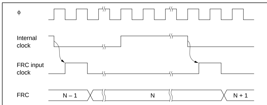
Figure 11.3 Increment Timing with Internal Clock Source
