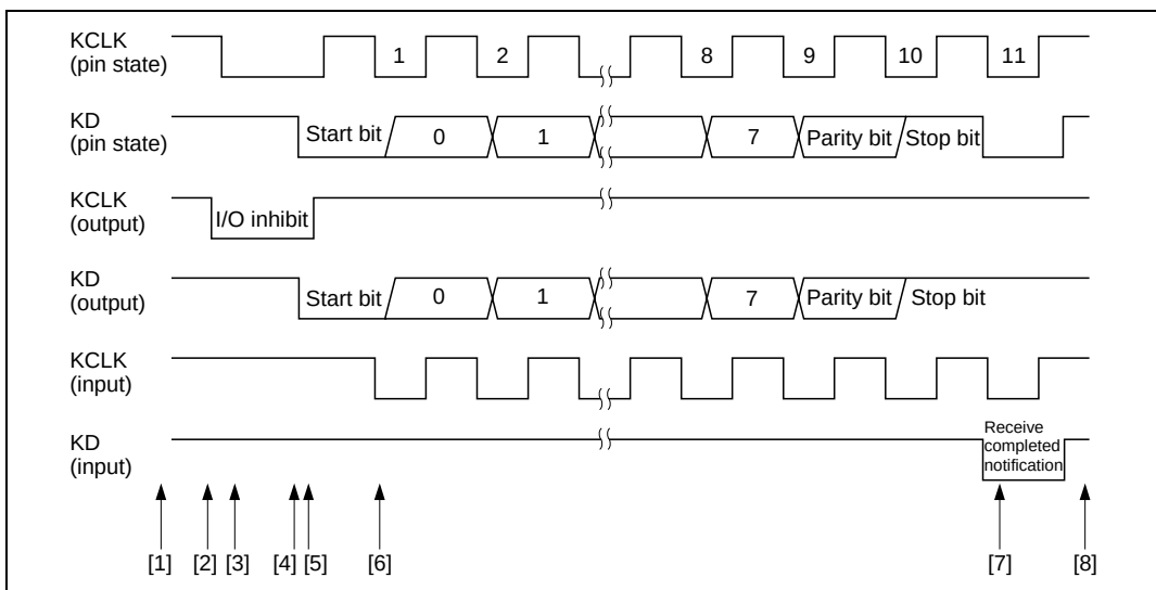
Figure 17.6 Transmit Timing
