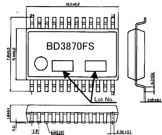
SSOP-A24 (Unit: mm)
