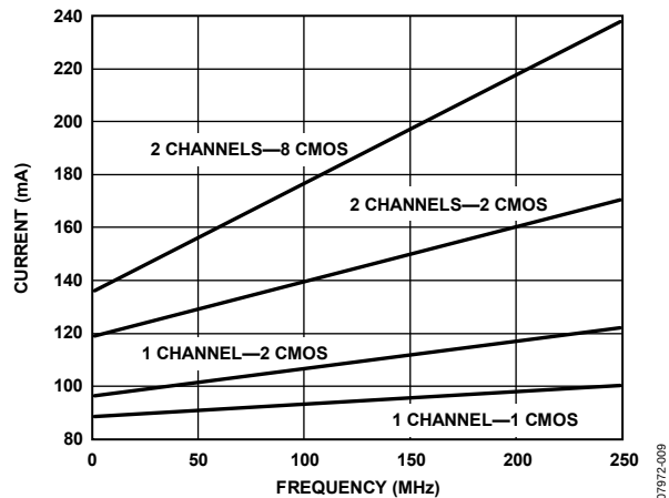
Figure 9. Current vs. Frequency—CMOS Outputs with 10 pF Load
