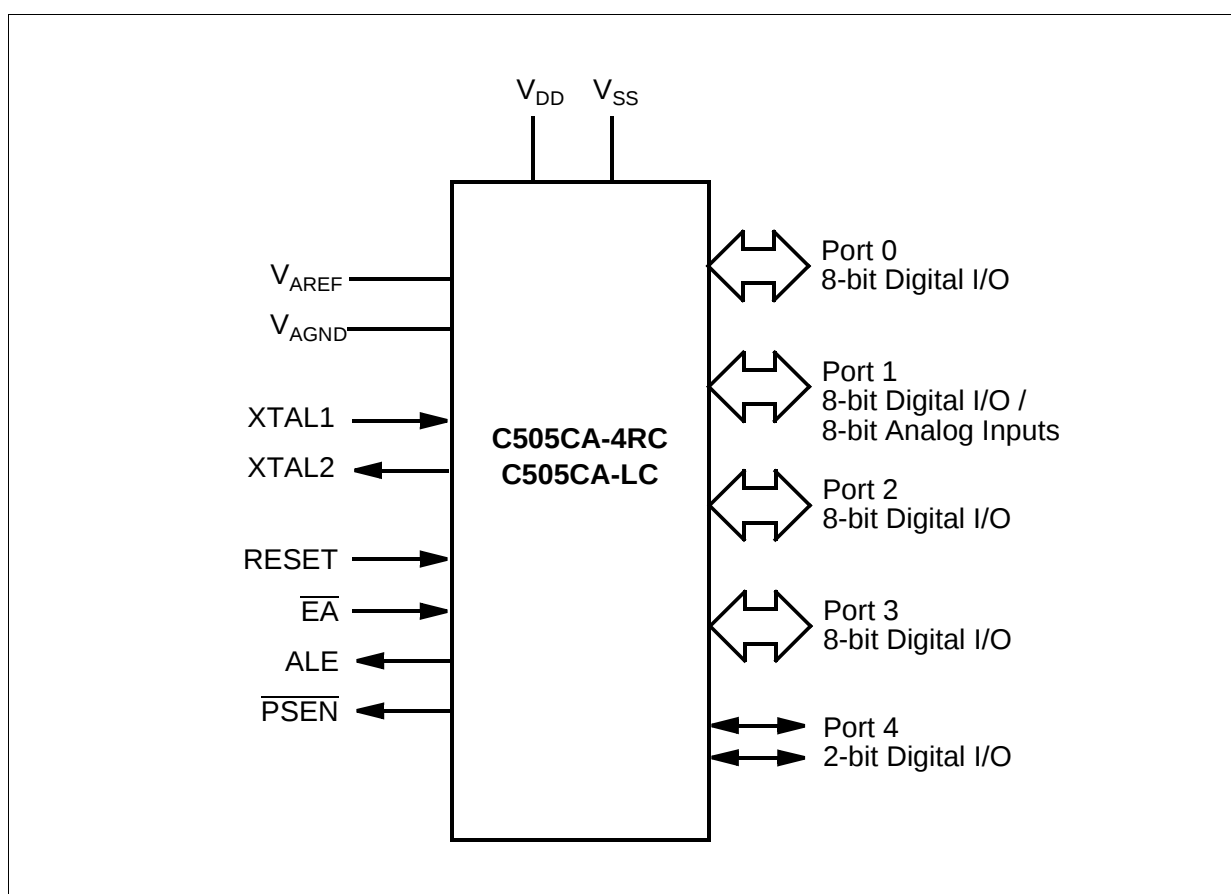
Figure 2 Logic Symbol
