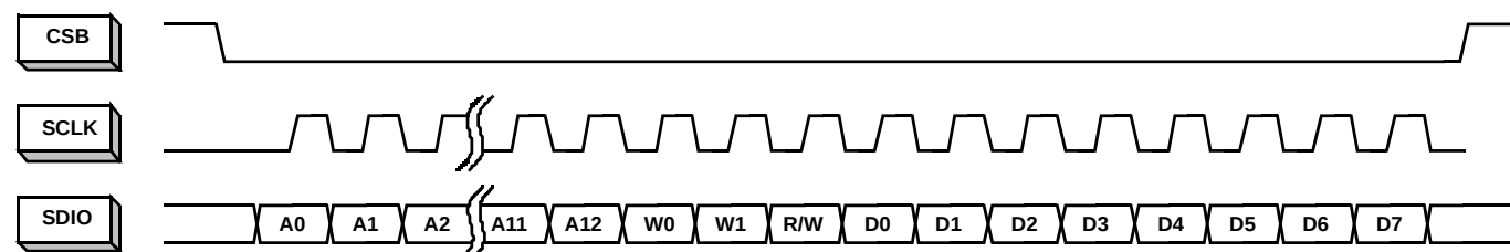
FIGURE 53. LSB-FIRST ADDRESSING
