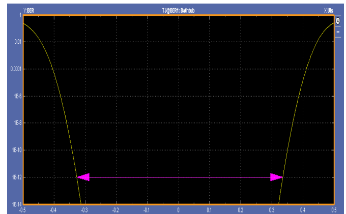
FIGURE 30. SERDES BATHTUB at 4.375Gbps
