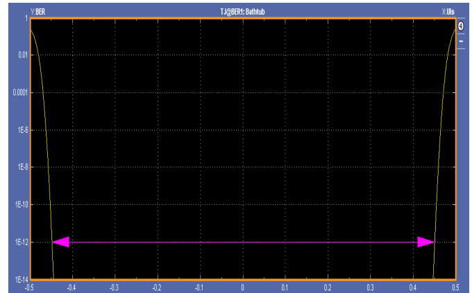
FIGURE 28. SERDES BATHTUB at 1.0Gbps
