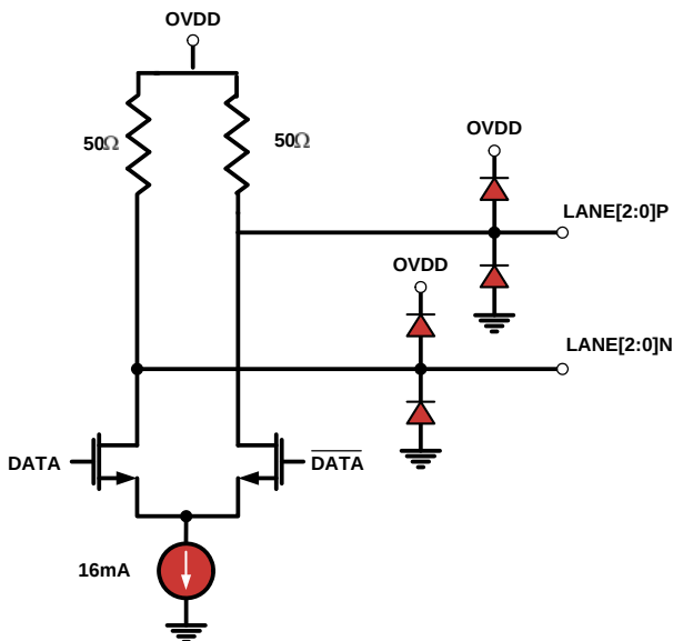
FIGURE 62. CML OUTPUTS
