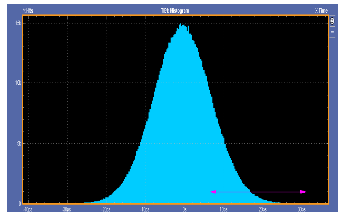
FIGURE 32. SERDES HISTOGRAM at 3.0Gbps
