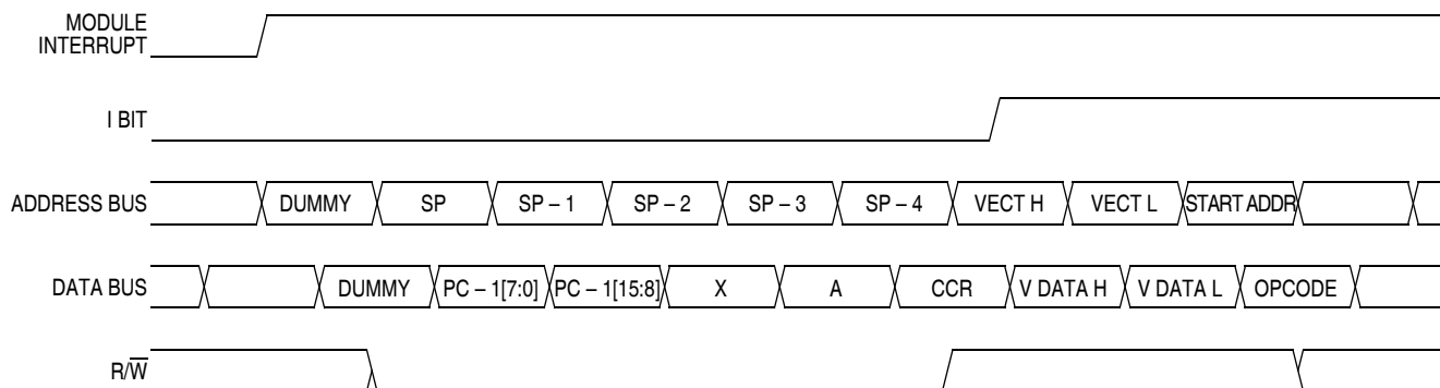
Figure 13-8. Interrupt Entry
