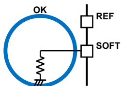
Resistor Pull-down
