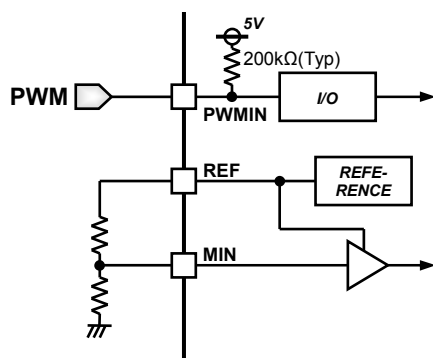
Figure 17. PWM input and minimum output duty setting
