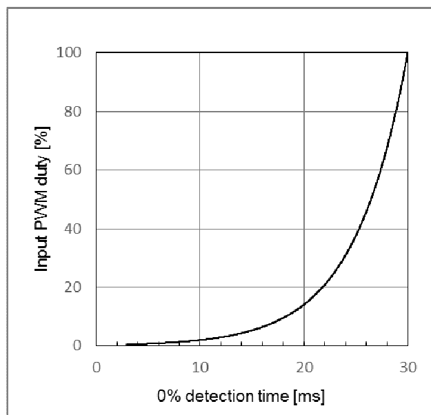
Figure 39. Input PWM DUTY vs 0% detection time
