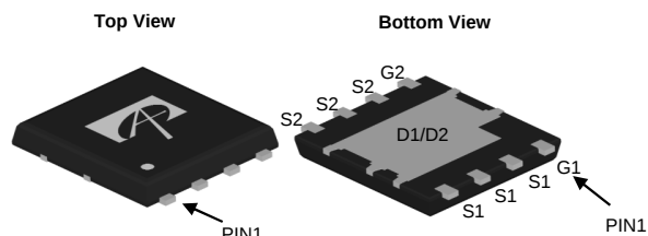
DFN5X6B
