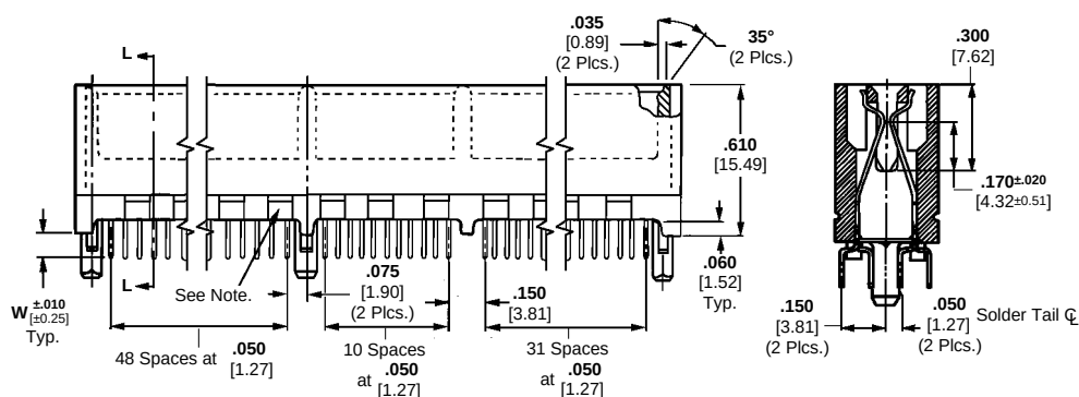
Section L-L
