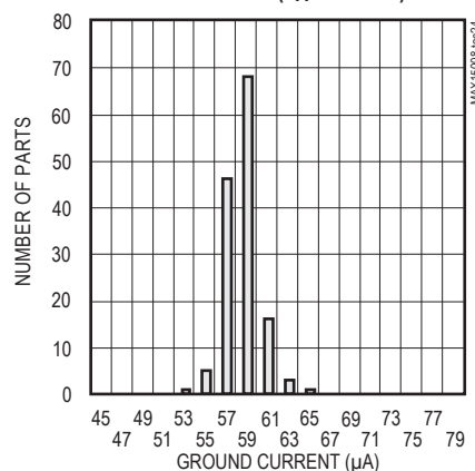
GROUND CURRENT DISTRIBUTION HISTOGRAM ( T_A = +125^\circ C )
