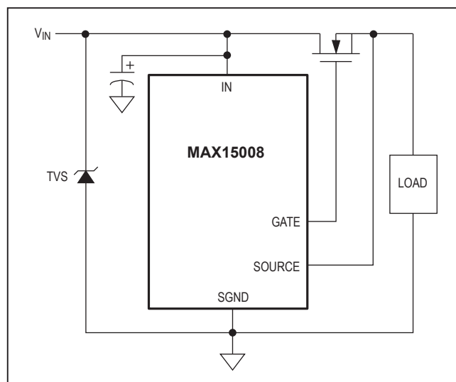
Figure 6. Protecting the MAX15008 Input from High-Voltage Transients
