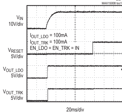
STARTUP RESPONSE THROUGH V_{IN}
