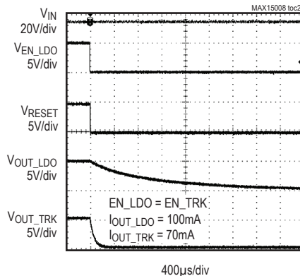
SHUTDOWN RESPONSE THROUGH EN
