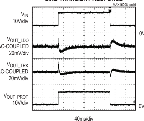
LINE-TRANSIENT RESPONSE
