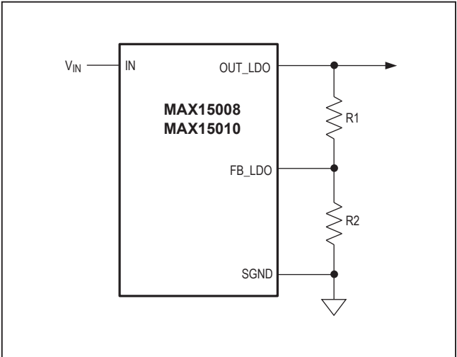
Figure 3. Setting the LDO Output Voltage
