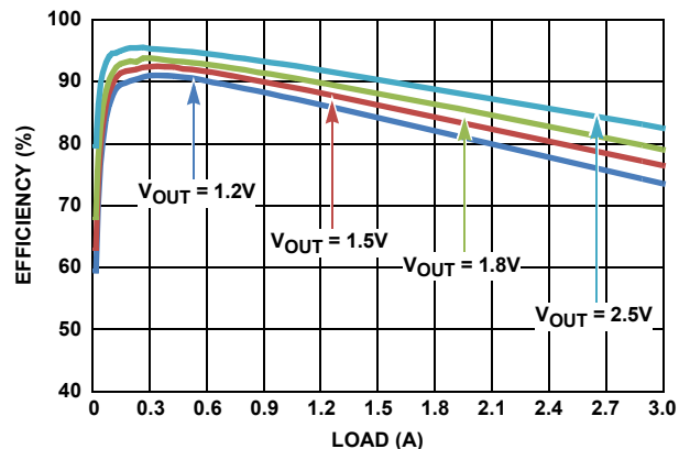
FIGURE 5. EFFICIENCY vs LOAD (ISL80030A) f_{SW} = 2\text{MHz} , V_{IN} = 3.3\text{V} , PWM, T_A = +25^\circ\text{C}
