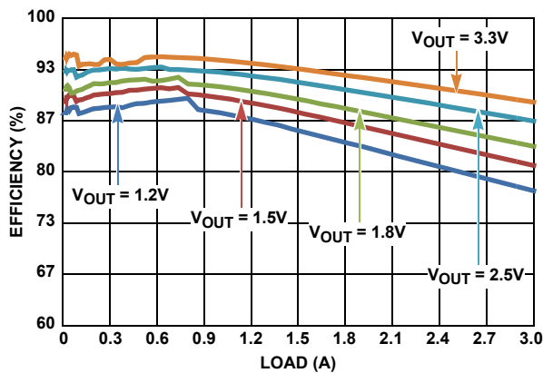
FIGURE 8. EFFICIENCY vs LOAD (ISL80031A) f_{SW} = 2\text{MHz} , V_{IN} = 5\text{V} , PFM, T_A = +25^\circ\text{C}
