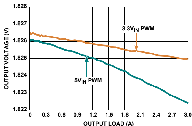
FIGURE 13. V_{OUT} REGULATION vs LOAD (ISL80030) f_{SW} = 1\text{MHz} , V_{OUT} = 1.8\text{V} , PWM, T_A = +25^\circ\text{C}
