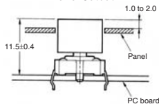
Panel Cutout
