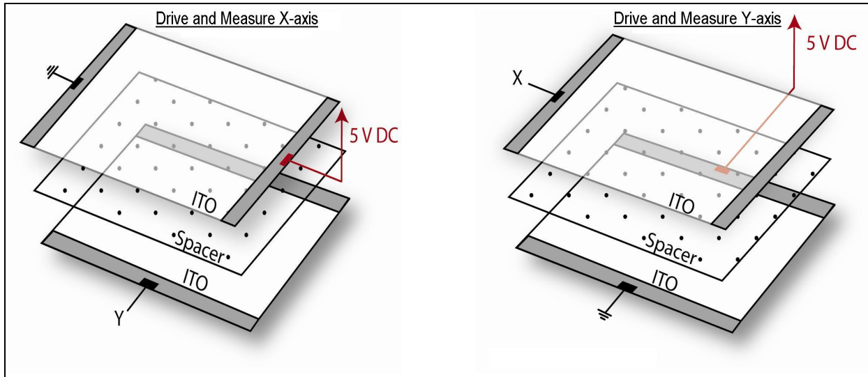
FIGURE 2-1: 4-WIRE DECODING
