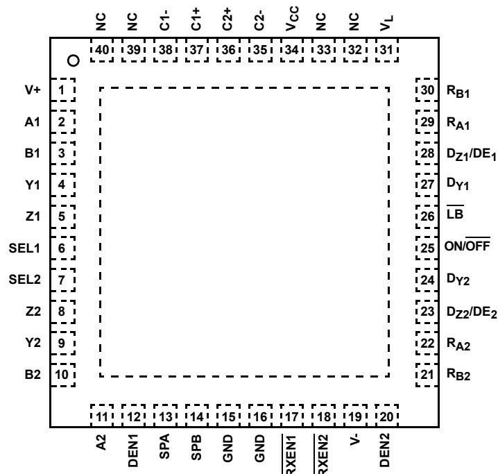
ISL3333 (40 LD QFN) TOP VIEW
