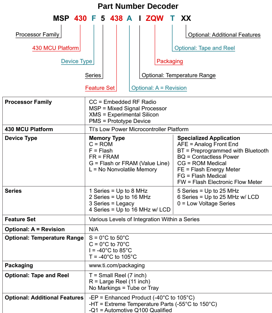
Figure 2. Device Nomenclature
