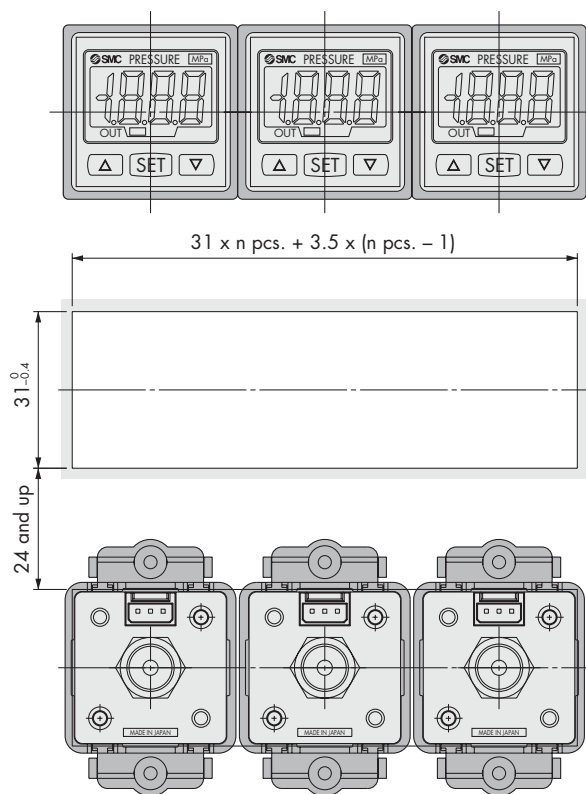
Multiple (2 pcs. or more) horizontal mounting
