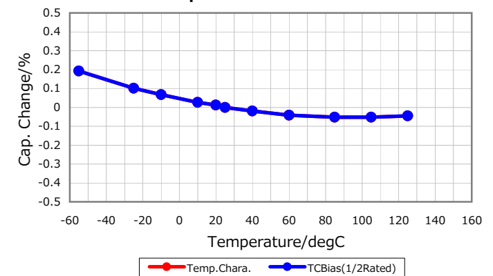
Temperature Characteristic
