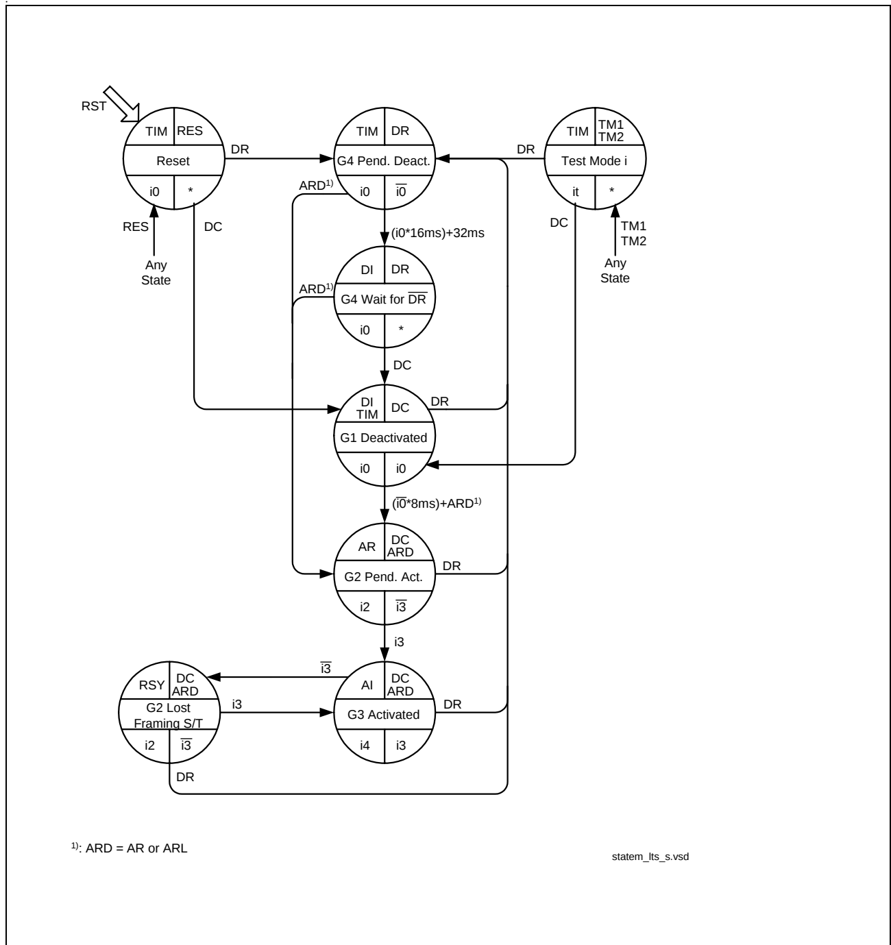
Figure 56 State Machine LT-S Mode
