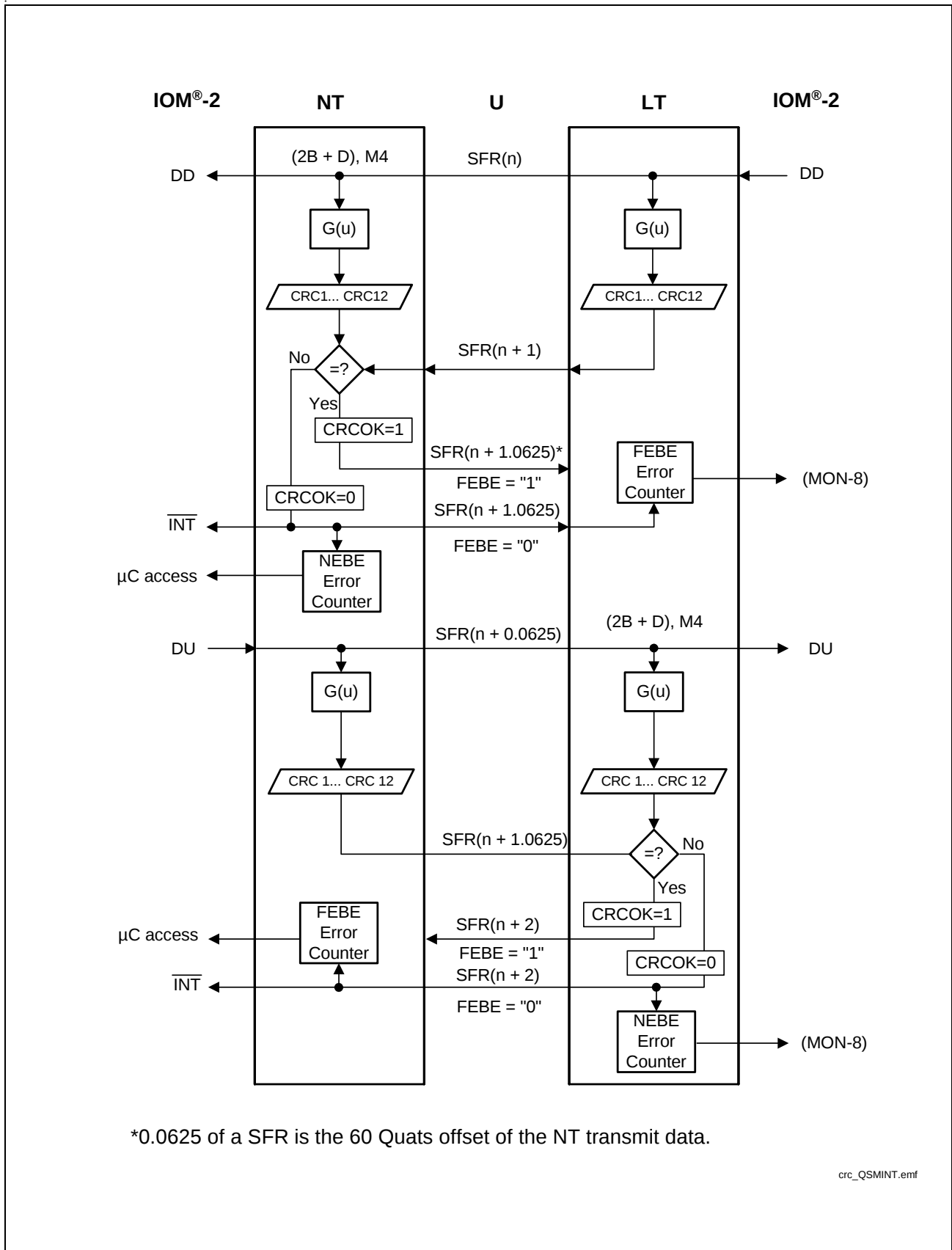
Figure 44 CRC-Process
