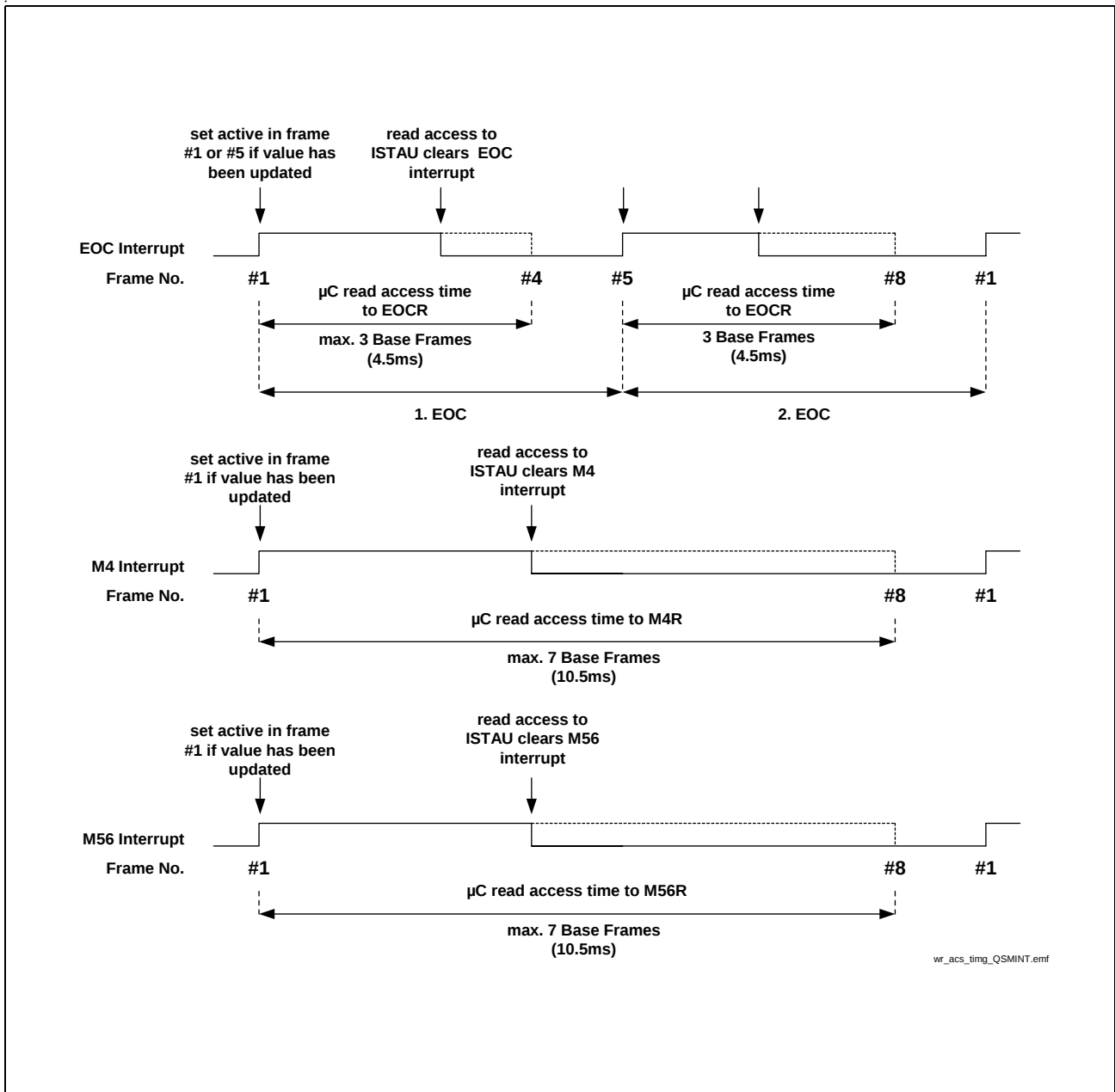
Figure 37 Read Access Timing
