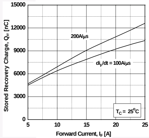
Figure 20. Stored Charge
