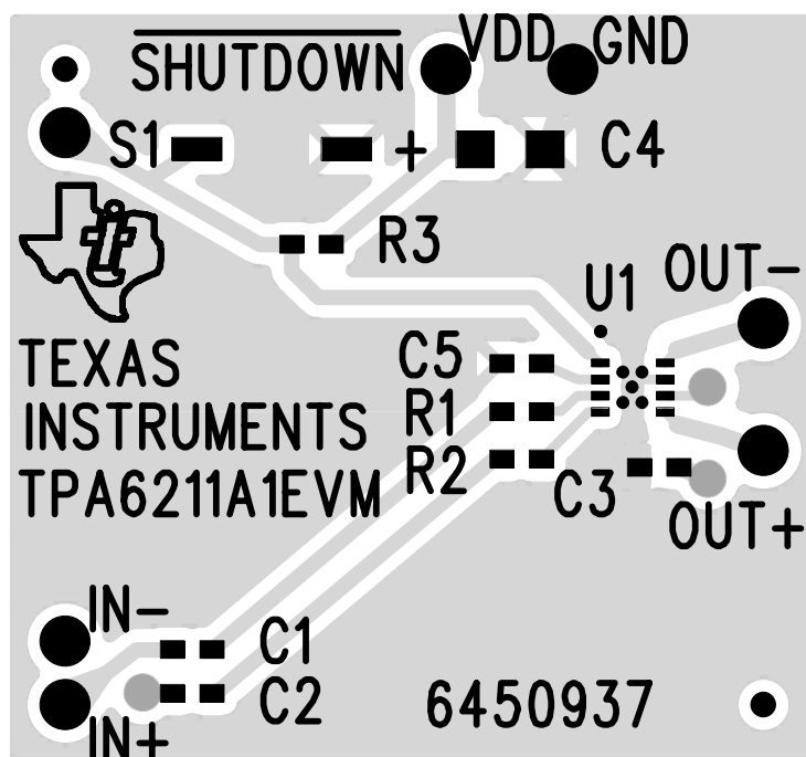
Figure 1–1. TI TPA6211A1 Audio Amplifier Evaluation Module
