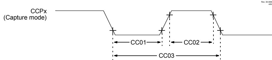
Figure 40-13. Capture/Compare/PWM Timings (CCP)
