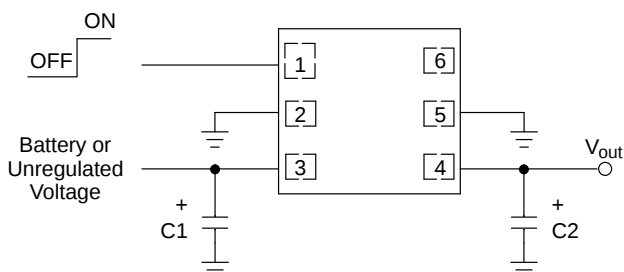
Figure 28. Typical Application Circuit
