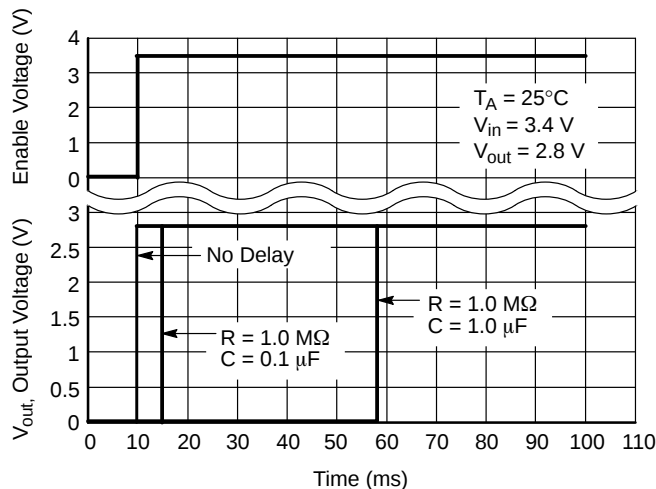
Figure 33. Delayed Turn-on
